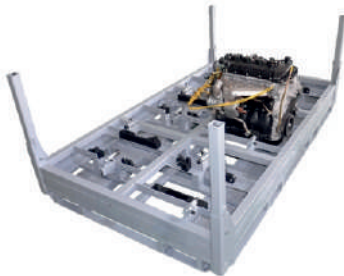
ENGINE AND TRANSMISSION STORAGE PALLET
